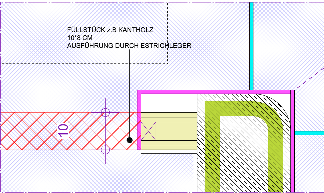
POS.2 M1:5
